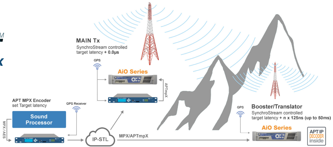
APT SynchroStream achieves perfect and dynamic compensation of IP link latencies and manages modulation timing
