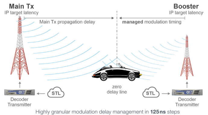
Highly granular modulation delay management in 125ns steps
