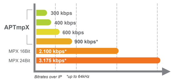
Data rates of linear MPX and compressed APTmpX
