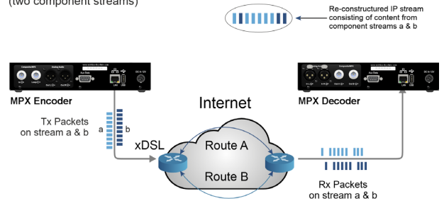
xDSL connections become the broadcast links
